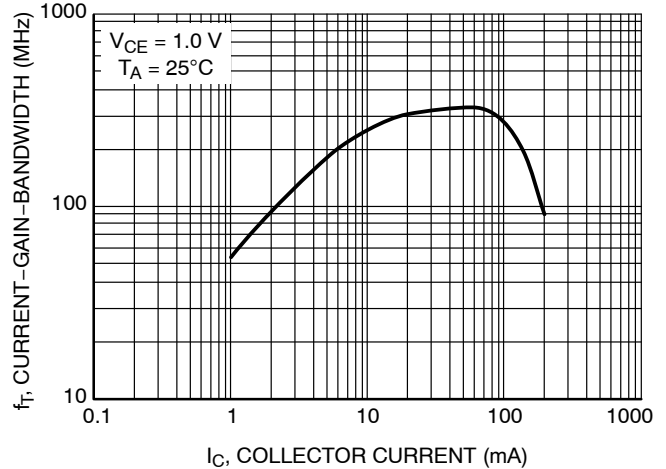
Figure 21. Current-Gain-Bandwidth Product
