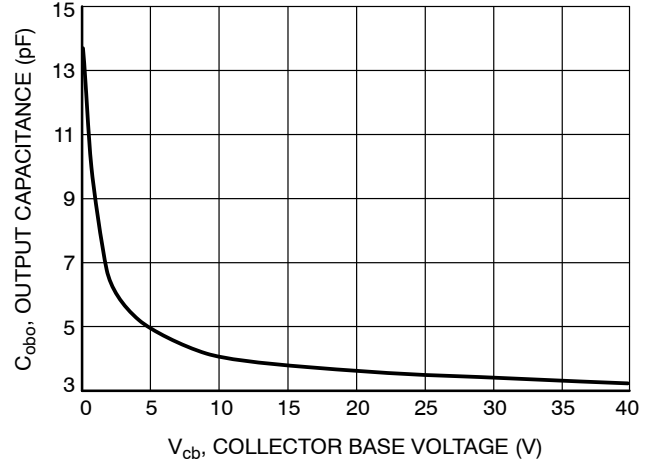
Figure 19. Output Capacitance vs. Collector Base Voltage
